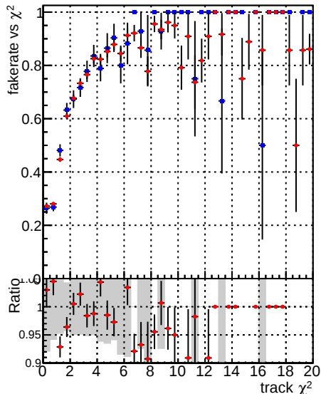
Fake rate vs. \chi^2 for different seeders
