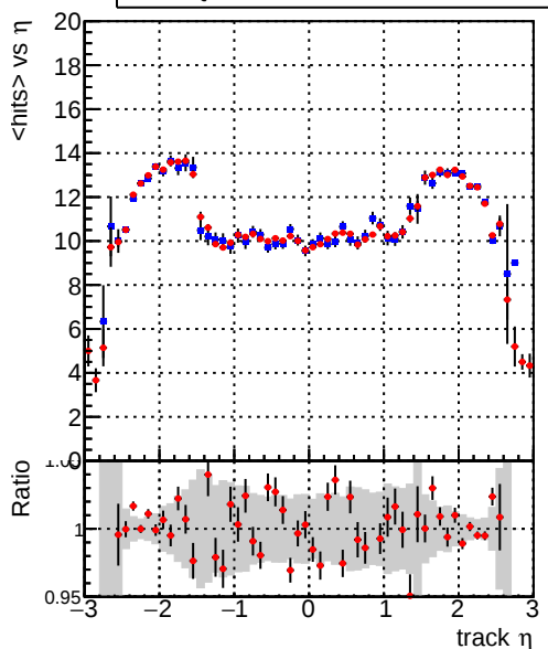
mean hit Legend: DQM_mkFit_TTbase (blue line), DQM_mkFit_TTtest125xNEW (red line)
