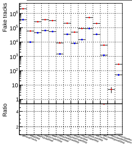
Number —●— DQM_mkFit_TTtest125xNEW
