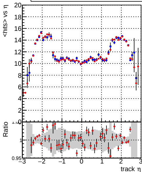
mean hits — DQM_mkFit_TTbase — DQM_mkFit_TTtest125xNEW
