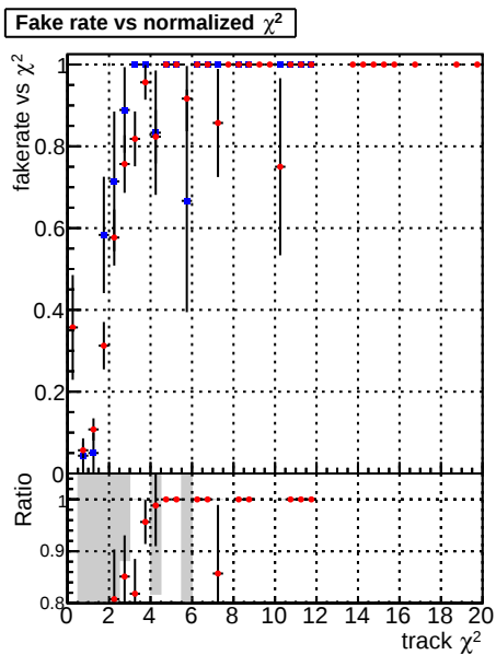
Fake rate vs. —●— DQM_mkFit_TTbase —●— DQM_mkFit_TTtest125xNEW
