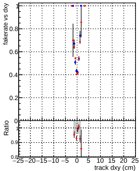
—●— DQM_mkFit_TTbase —●— DQM_mkFit_TTtest125xNEW
