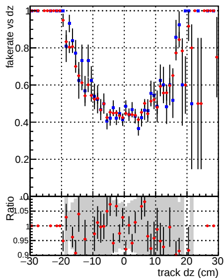
—●— DQM_mkFit_TTbase —●— DQM_mkFit_TTtest125xNEW
