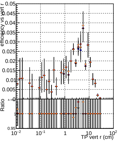
Efficiency vs TP vert r (cm) —●— DQM_V0001_R000000001 Global mkFitOriginal RECO —●— DQM_V0001_R000000001 Global mkFitNewDet RECO —●— DQM_V0001_R000000001 Global mkFitNewDet33 RECO —●— DQM_V0001_R000000001 Global mkFitNewDetNoF RECO
