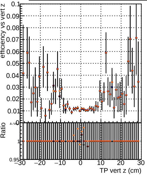
Efficiency vs vertpos —●— DQM_V0001_R0000000001 Global mkFitOriginal RECO —●— DQM_V0001_R0000000001 Global mkFitNewDett RECO —●— DQM_V0001_R0000000001 Global mkFitNewDett33 RECO —●— DQM_V0001_R0000000001 Global mkFitNewDettNoF RECO
