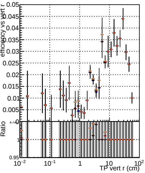
Efficiency vs vertpos —●— DQM_V0001_R000000001 Global mkFitOriginal RECO —●— DQM_V0001_R000000001 Global mkFitNewDett RECO —●— DQM_V0001_R000000001 Global mkFitNewDett33 RECO —●— DQM_V0001_R000000001 Global mkFitNewDettNoF RECO
