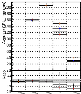
detachedTripletStep
