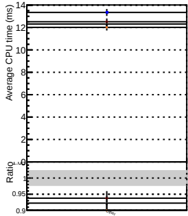
generalTracks
