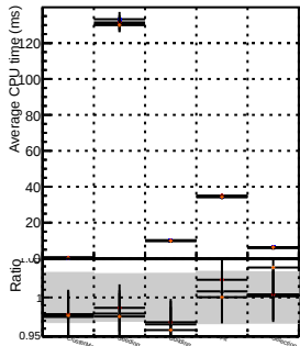
detachedQuadStep
