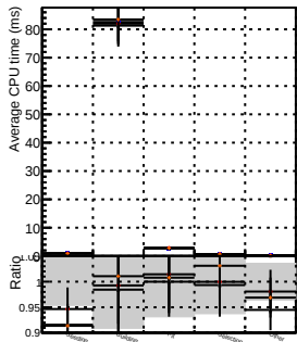
jetCoreRegionalStep
