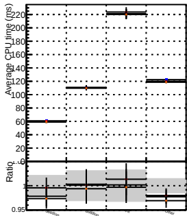
InitialStepPreSplitting
