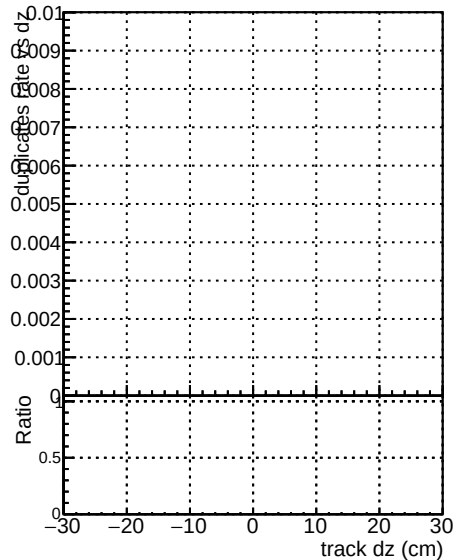
Global fit New Belle II RECO
