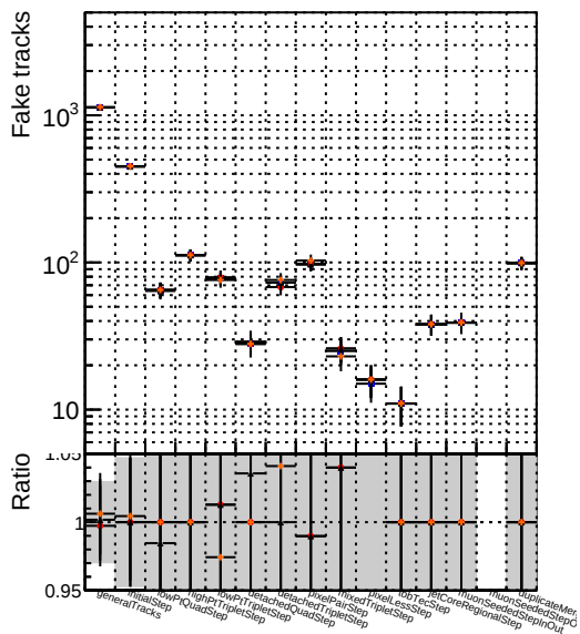
Number DOM V0001 R0000000001 Global mkFitNewDet33 RECO DOM V0001 R0000000001 Global mkFitNewDetNoF RECO
