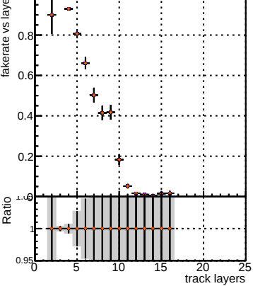
Fake rate vs layer
