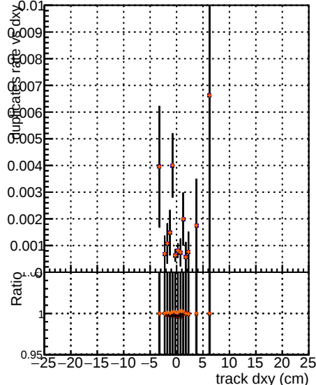
Global mkFit Original RECO Global mkFit NewDet32 RECO Global mkFit NewDet32 RECO
