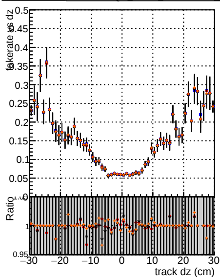
Global mkFit Original RECO Global mkFit NewDet32 RECO Global mkFit NewDet32 RECO
