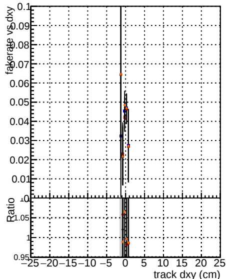
Legend for Fake rate vs dxy, Duplicates Rate vs Dxy, and Pileup rate vs dxy: Global (black line) mkFit (blue line) Original (red line) RECO (orange line)
