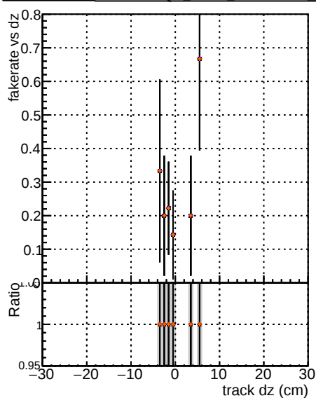
Fake rate vs d DGM V0001 B0000000001 Global mkFitOriginal RECO DGM V0001 B0000000001 Global mkFitNewDet133 RECO DGM V0001 R0000000001 Global mkFitNewDet104 RECO
