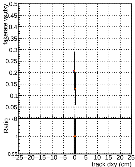
Fake rate vs d DGM V0001 B0000000001 Global mkFitOriginal RECO DGM V0001 B0000000001 Global mkFitNewDet133 RECO DGM V0001 R0000000001 Global mkFitNewDet104 RECO
