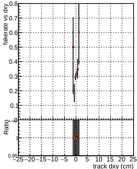
Fake rate vs d DQM V0001 B00000000001 Global mkFitOriginal RECO DQM V0001 B00000000001 Global mkFitNewDet133 RECO DQM V0001 B00000000001 Global mkFitNewDet104 RECO
