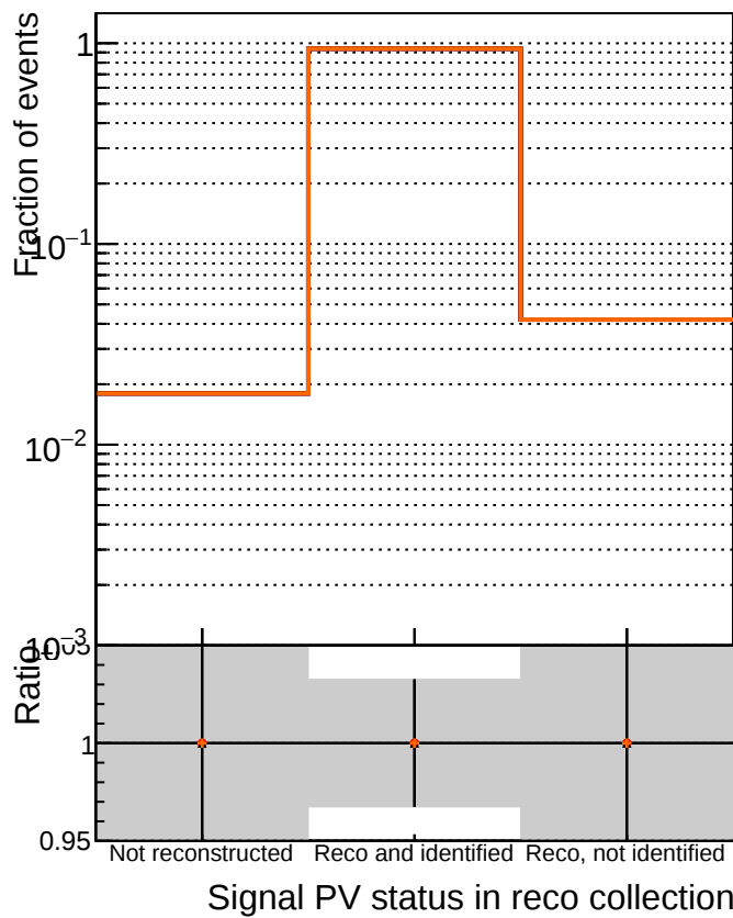
TruePVLocationIndexInRecoVertexCollectionCumulative
