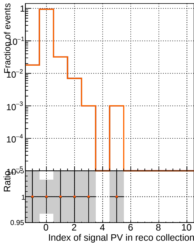
TruePVLocationIndexInRecoVertexCollection
