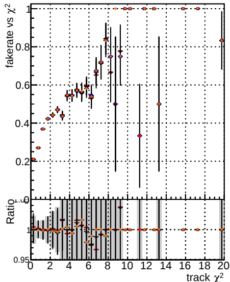
Fake rate vs. \chi^2 vs seeding layers
