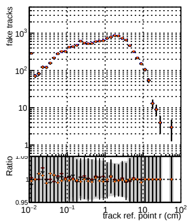
N of associated (recoToSim) fake tracks vs transverse ref point position
