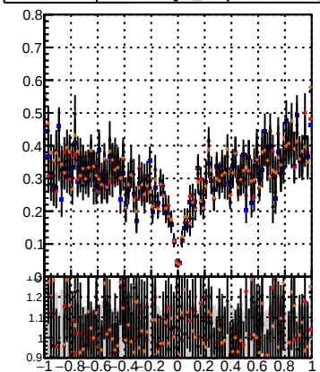
— DOM DisplacedSUSY CKF — DOM DisplacedSUSY mkFit — DOM DisplacedSUSY CKF BDT — DOM DisplacedSUSY mkFit BDT
