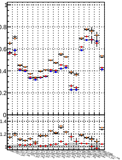
Fake rate vs. —●— BDM Displaced SUSY CKFit —+— Displaced SUSY CKFit BDT
