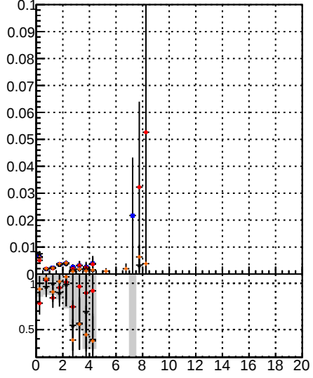
Fake rate vs. —●— BDM Displaced SUSY CKFit —+— Displaced SUSY CKFit BDT
