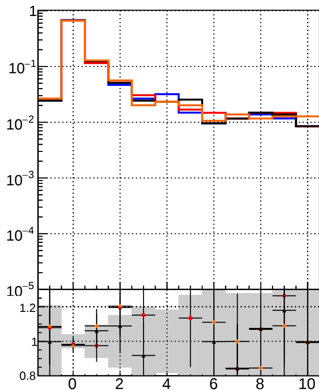
TruePVLocationIndexInRecoVertexCollection
