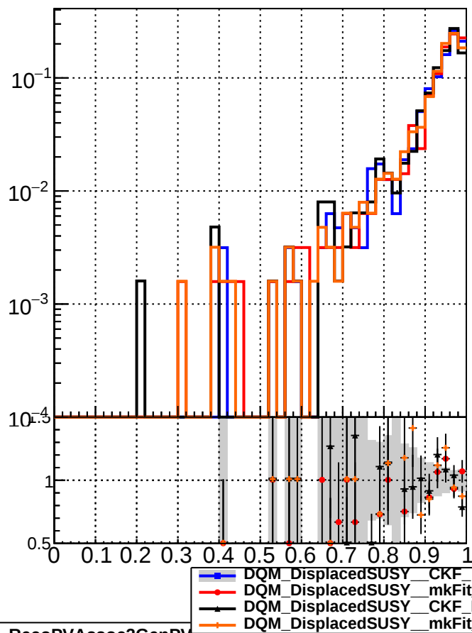
RecoPVAssoc2GenPVMatched_missing
