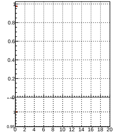
Fake rate vs. \chi^2 for various models and fits. Legend: DOM Displaced SUSY CKE Fit, DOM Displaced SUSY CKE Fit BDT, DOM Displaced SUSY CKE Fit BDT.
