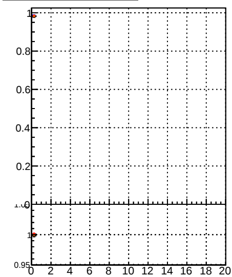
Fake rate vs. \chi^2 for BDT, CKF, and BDT+CKF. Legend: BDT (blue), Displaced SUSY (orange), CKF (red), BDT+CKF (black).
