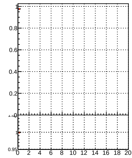
Fake rate vs. \chi^2 for BSM Displaced SUSY CKE Fit, BDT, and CKFit
