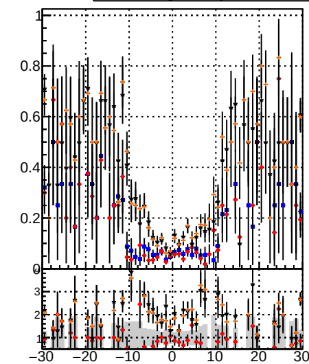
—●— DQM Displaced SUSY CKFit —●— DQM Displaced SUSY CKFit_BDT —●— DQM Displaced SUSY CKFit_BDT
