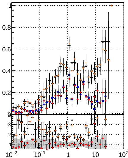
—●— DQM Displaced SUSY CKFit —●— DQM Displaced SUSY CKFit_BDT —●— DQM Displaced SUSY CKFit_BDT
