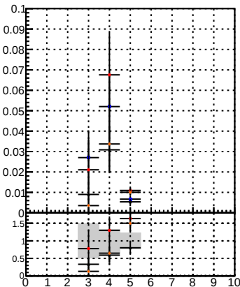
kFit_BDT_
