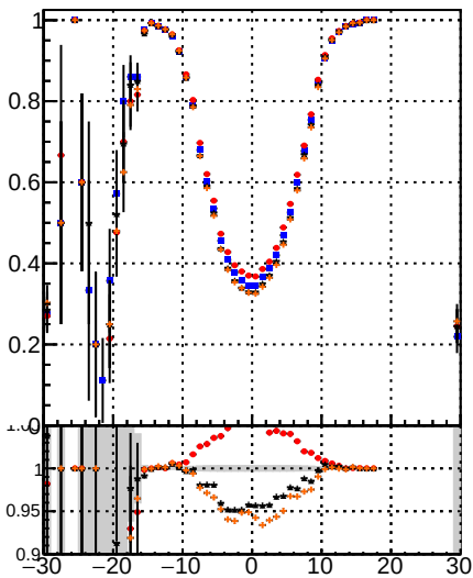
Fake rate vs v DOM Displaced SUSY CKFit CKFit+BDT CKFit+BDT
