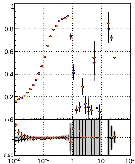
DOM Displaced SUSY CKE DOM Displaced SUSY CKEfit DOM Displaced SUSY mKEfit DOM Displaced SUSY mKEfit BDT
