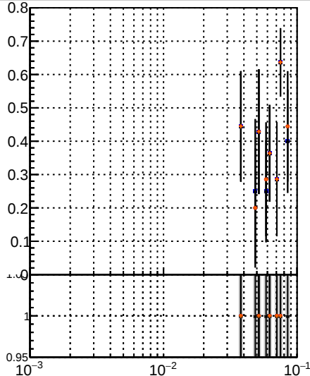
\frac{E_{it}^{BDT}}{E_{it}^{BDT}}
