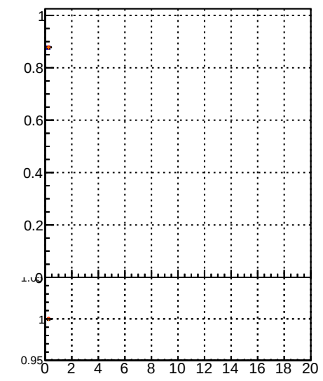
Fake rate vs. \chi^2 for various models and fits. Legend: BSM Displaced SUSY (blue), BSM Displaced SUSY CKFit (red), BSM Displaced SUSY CKFit BDT (orange), BSM Displaced SUSY CKFit BDT (green).
