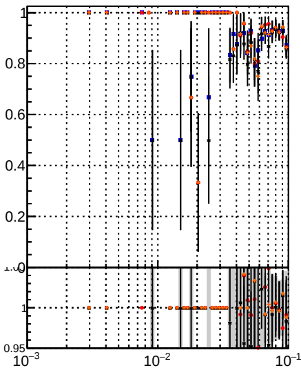
Fake rate vs \frac{1}{\text{dr}} Legend: DOM Displaced SUSY CKE DOM Displaced SUSY CKEfit DOM Displaced SUSY CKEfit BDT DOM Displaced SUSY mkFit BDT
