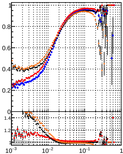
Fake rate vs \frac{1}{\text{dr}} Legend: DOM Displaced SUSY CKE DOM Displaced SUSY CKEfit DOM Displaced SUSY CKEfit BDT DOM Displaced SUSY mkFit BDT
