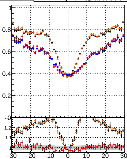
—●— DOM Displaced SUSY CKE —●— DOM Displaced SUSY CKE fit —●— DOM Displaced SUSY BDT —●— DOM Displaced SUSY mKE fit BDT
