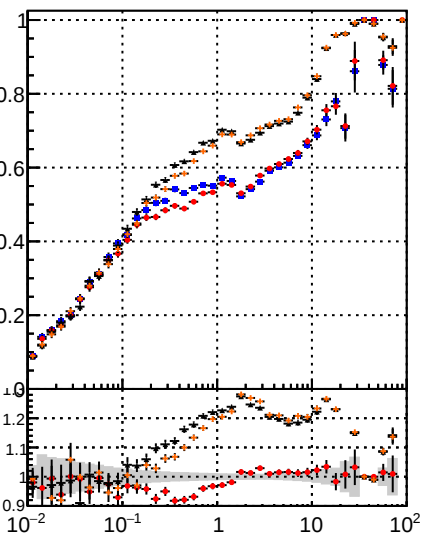
—●— DOM Displaced SUSY CKE —●— DOM Displaced SUSY CKE fit —●— DOM Displaced SUSY BDT —●— DOM Displaced SUSY mKE fit BDT
