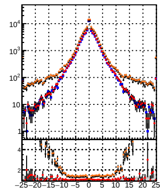
—●— DOM Displaced SUSY CKE —●— DOM Displaced SUSY mke-it BDT —●— DOM Displaced SUSY mke-it BDT
