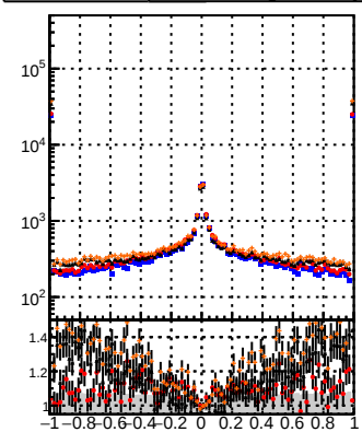
—●— DOM Displaced SUSY CKE —●— DOM Displaced SUSY mke-it BDT —●— DOM Displaced SUSY mke-it BDT
