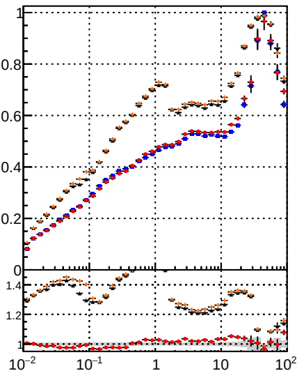
Fake rate vs \nu DOM Displaced SUSY CKE DOM Displaced SUSY CKE fit DOM Displaced SUSY mkFit BDT
