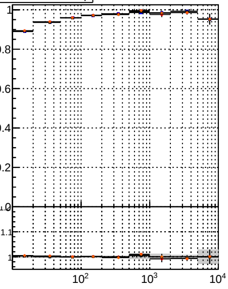
Efficiency vs Sum p_T^2
