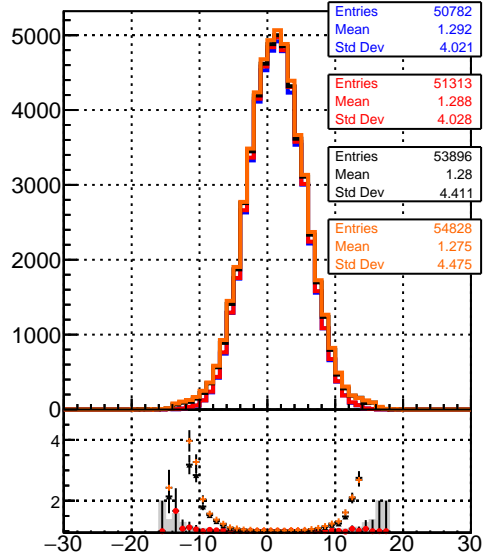
ReconstructedAllAssoc2Gen_NumTracks
