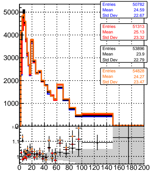
ReconstructedAllAssoc2Gen_NumTracks
