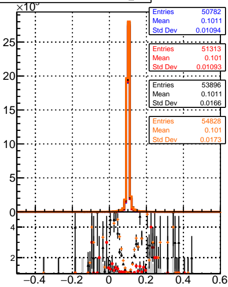
ReconstructedAllAssoc2Gen_X
