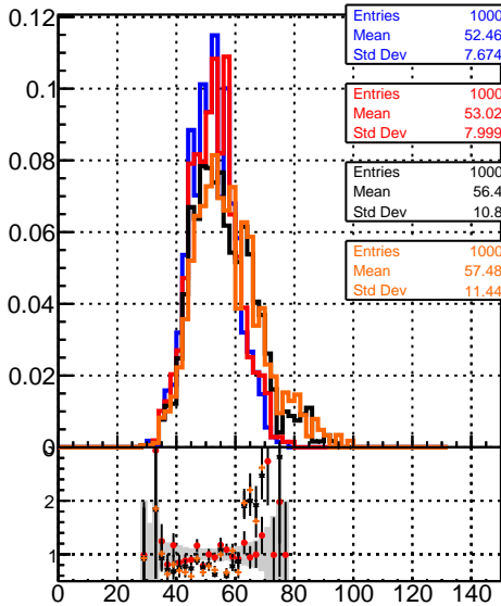
ReconstructedAllAssoc2Gen_NumVertices
