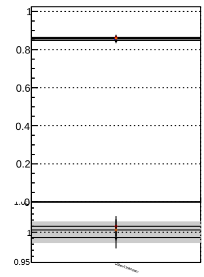
Fake rate vs. BSM Displaced SUSY CKFit BDT BSM Displaced SUSY CKFit BSM Displaced SUSY
