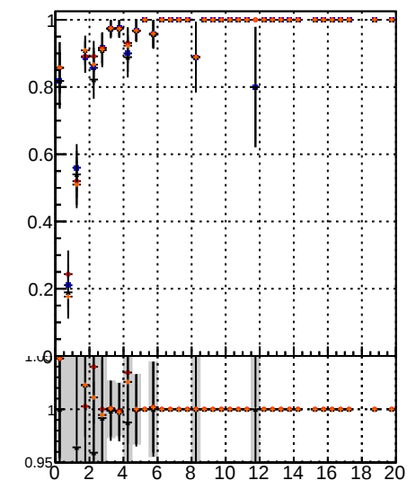
Fake rate vs. BSM Displaced SUSY CKFit BDT BSM Displaced SUSY CKFit BSM Displaced SUSY
