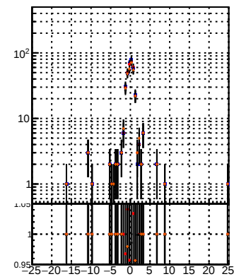
—●— DQM Displaced SUSY CKE —●— DQM Displaced SUSY CKE+BDT —●— DQM Displaced SUSY mke-fit BDT
