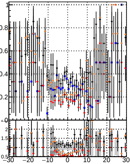
DOM Displaced SUSY CKE DOM Displaced SUSY CKE DOM Displaced SUSY CKE Fake rate vs vertpos Duplicates Rate vs vertpos Pileup rate vs vertpos
