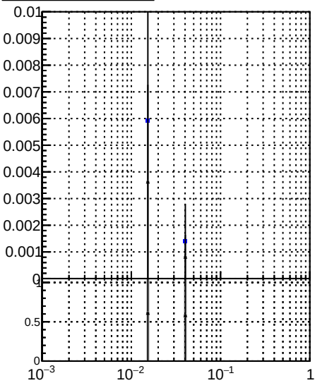
Fake rate vs DOM Displaced SUSY CKEfit DOM Displaced SUSY CKEfit BDT DOM Displaced SUSY mkFit BDT
