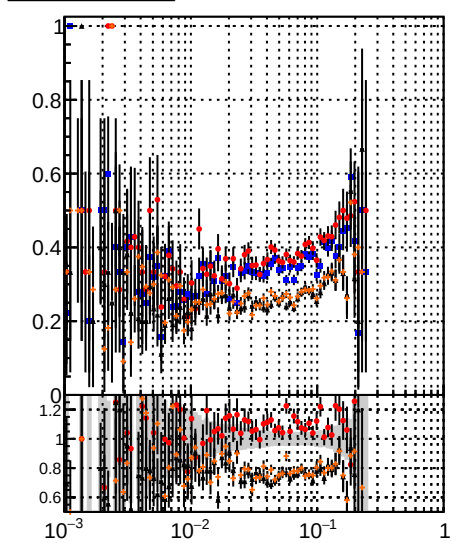
Fake rate vs DOM Displaced SUSY CKEfit DOM Displaced SUSY CKEfit BDT DOM Displaced SUSY mkFit BDT
