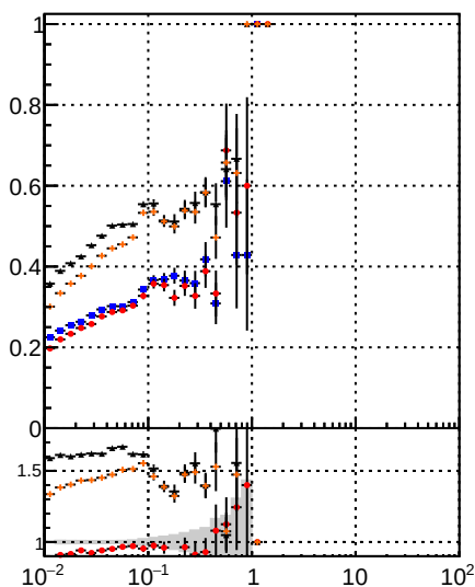
Fake rate vs v DOM Displaced SUSY CKE CKEfit BDT CKEfit+BDT
