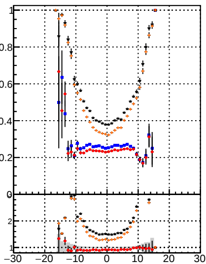
Fake rate vs d —●— BDT Displaced SUSY CKE Fit —●— BDT Displaced SUSY CKE Fit BDT —●— BDT Displaced SUSY CKE Fit BDT
