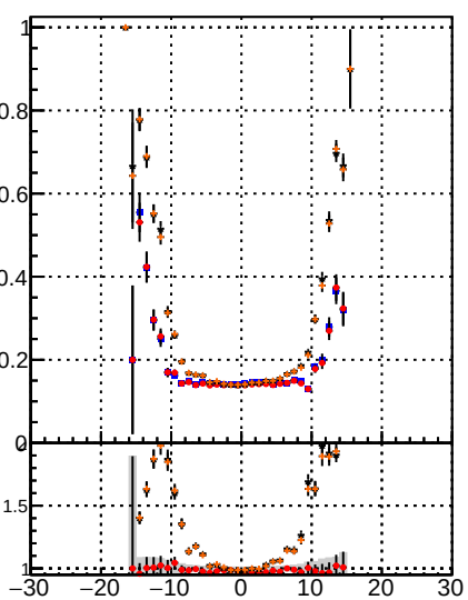
Fake rate vs d BSM Displaced SUSY CKFit BSM Displaced SUSY CKFit+BDT BSM Displaced SUSY CKFit+BDT
