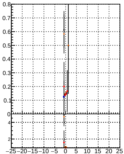
Fake rate vs d BSM Displaced SUSY CKFit BSM Displaced SUSY CKFit+BDT BSM Displaced SUSY CKFit+BDT
