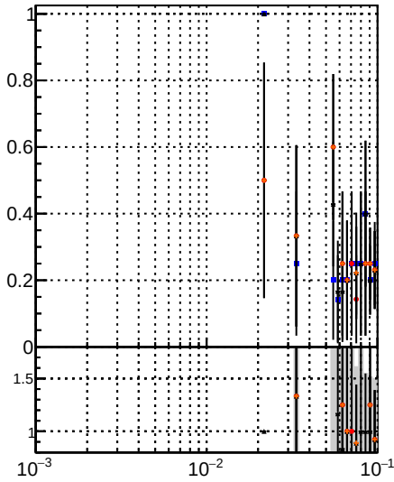
Fake rate vs \frac{dr}{\sqrt{s}} Legend: DOM (black line) Displaced SUSY (blue line) CKFit (red line) BDT (grey line)
