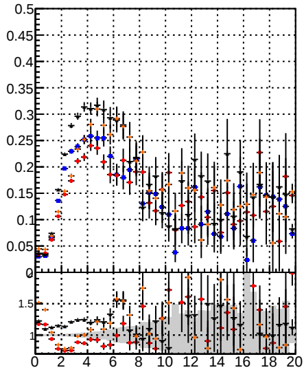
Fake rate vs. Model BDT BDM Displaced SUSY CKFit CKFit+BDT
