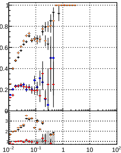
DOM Displaced SUSY CKE DOM Displaced SUSY CKE fit DOM Displaced SUSY mktFit BDT
