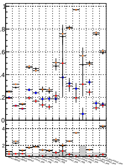
Fake rate vs. BDT Displaced SUSY CKFit BDT Displaced SUSY CKFit BDT Displaced SUSY CKFit
