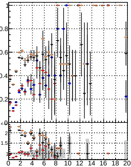
Fake rate vs. BDT Displaced SUSY CKFit BDT Displaced SUSY CKFit BDT Displaced SUSY CKFit
